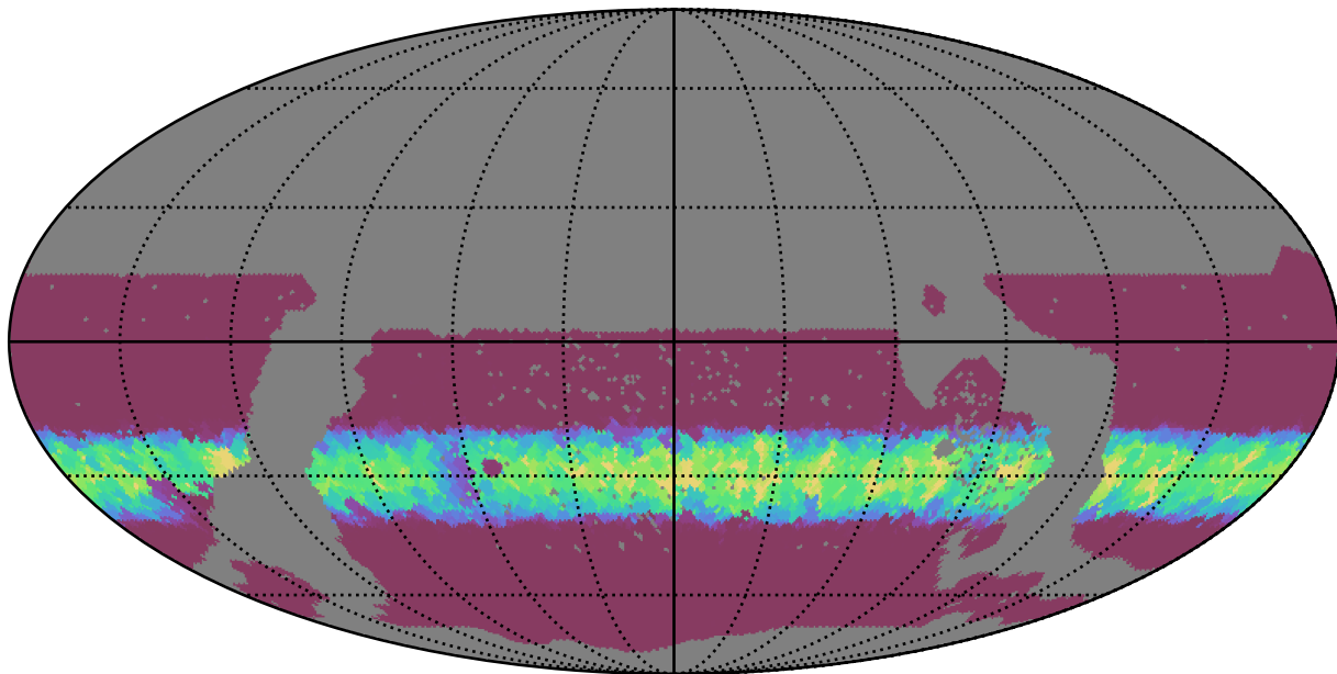
too_10_4v3.4_10yrs WFD z band: Min normairmass
