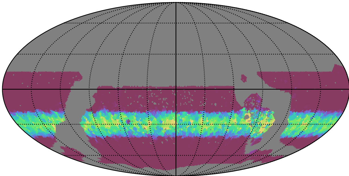
too_10_4v3.4_10yrs WFD u band: Min normairmass
