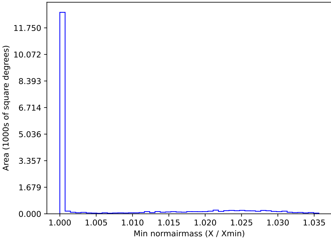
too_10_4v3.4_10yrs WFD r band: Min normairmass
