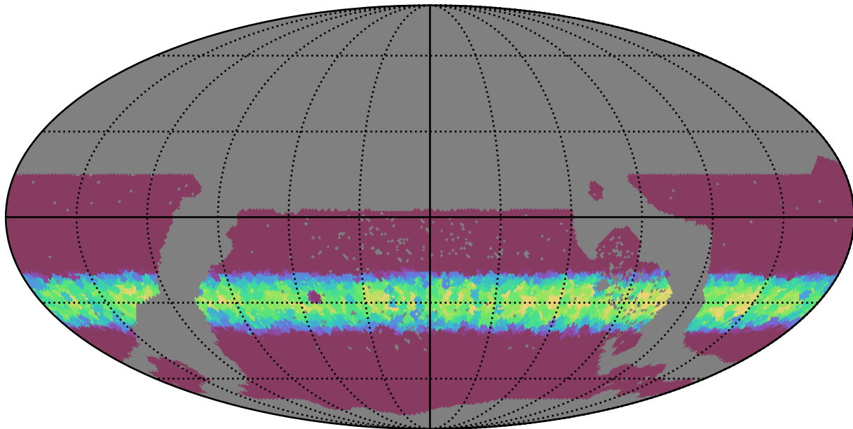
too_10_4v3.4_10yrs WFD i band: Min normairmass
