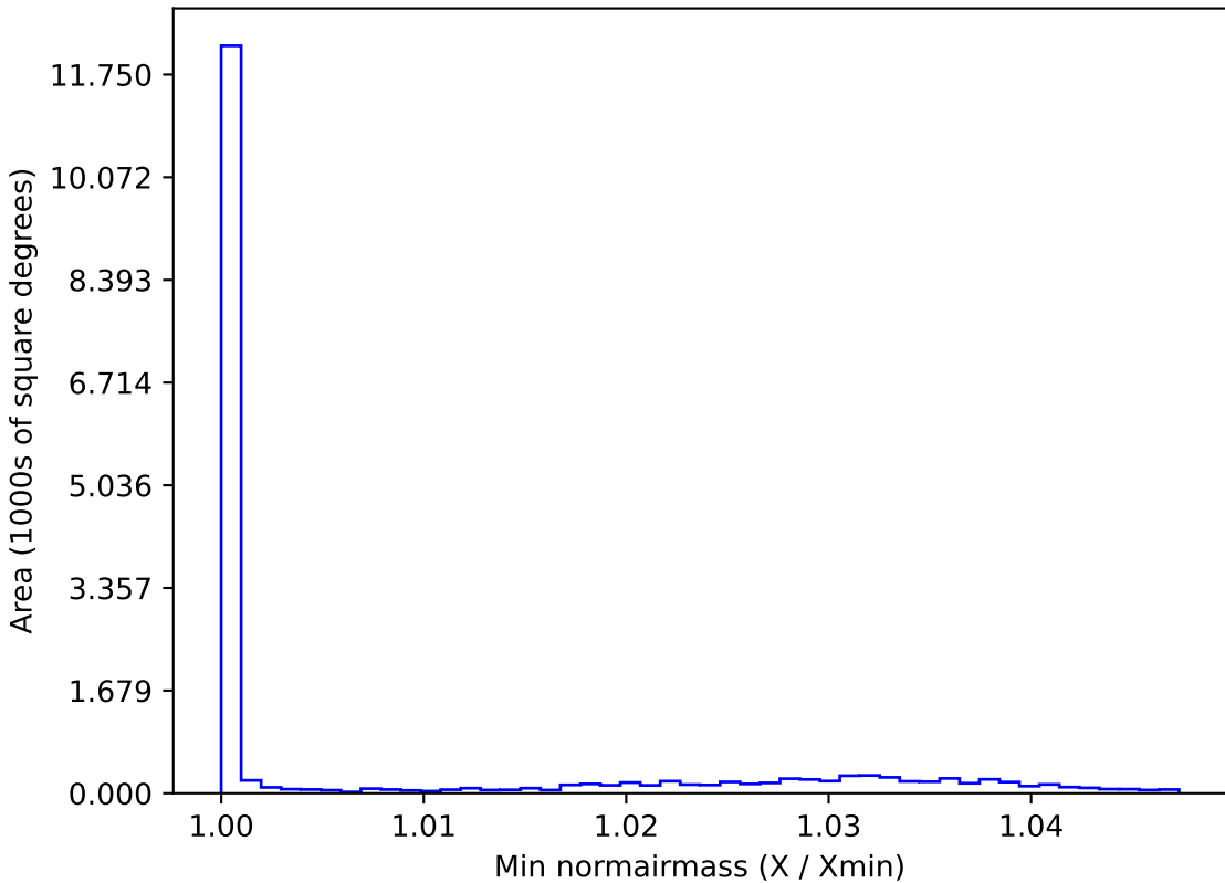
too_10_4v3.4_10yrs WFD g band: Min normairmass
