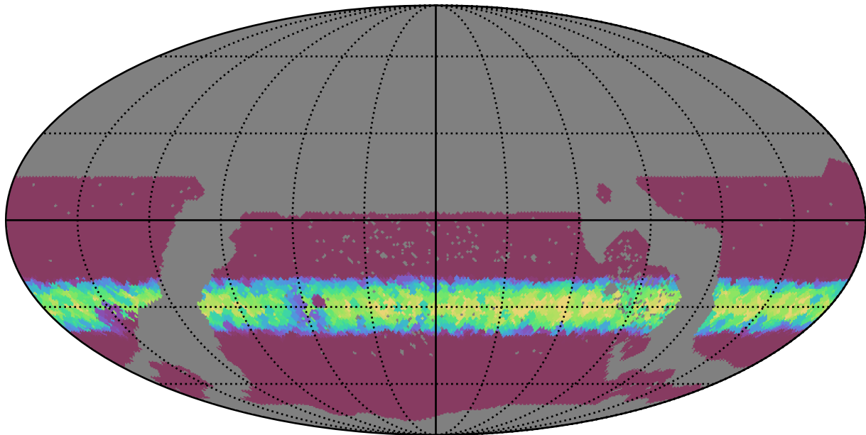
too_10_4v3.4_10yrs WFD all bands: Min normairmass
