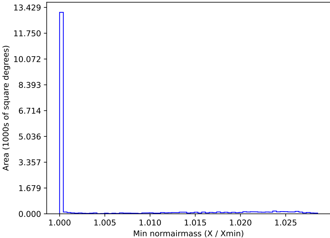
too_10_4v3.4_10yrs WFD all bands: Min normairmass
