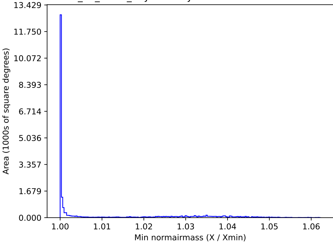
too_10_4v3.4_10yrs All sky u band: Min normairmass
