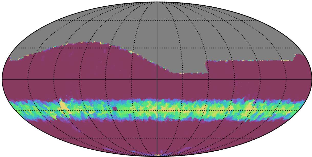
too_10_4v3.4_10yrs All sky r band: Min normairmass
