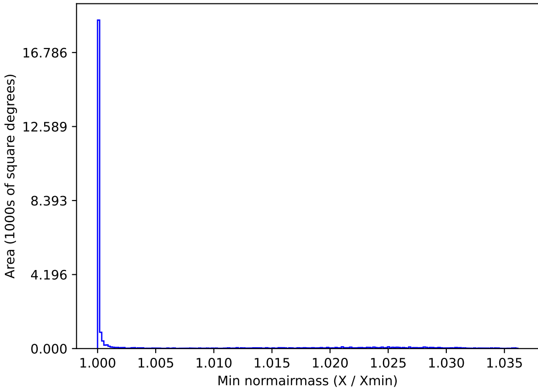
too_10_4v3.4_10yrs All sky r band: Min normairmass
