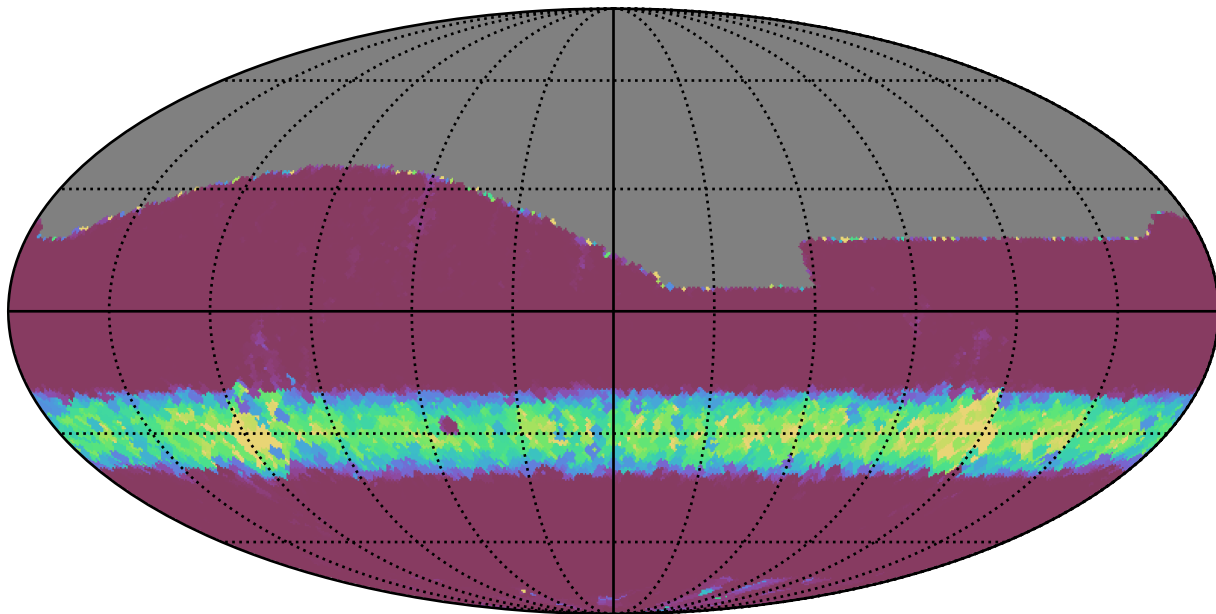
too_10_4v3.4_10yrs All sky i band: Min normairmass
