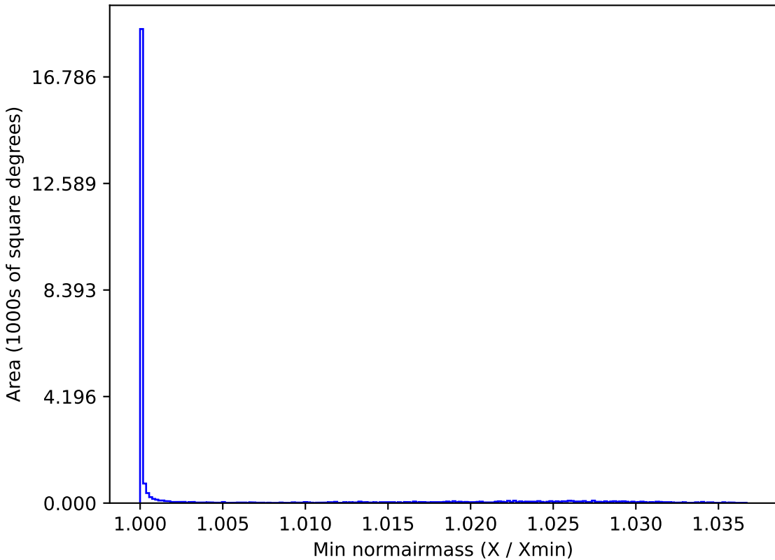
too_10_4v3.4_10yrs All sky i band: Min normairmass
