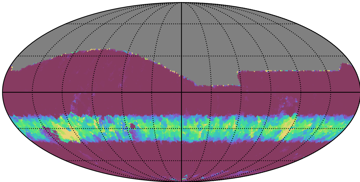
too_10_4v3.4_10yrs All sky g band: Min normairmass
