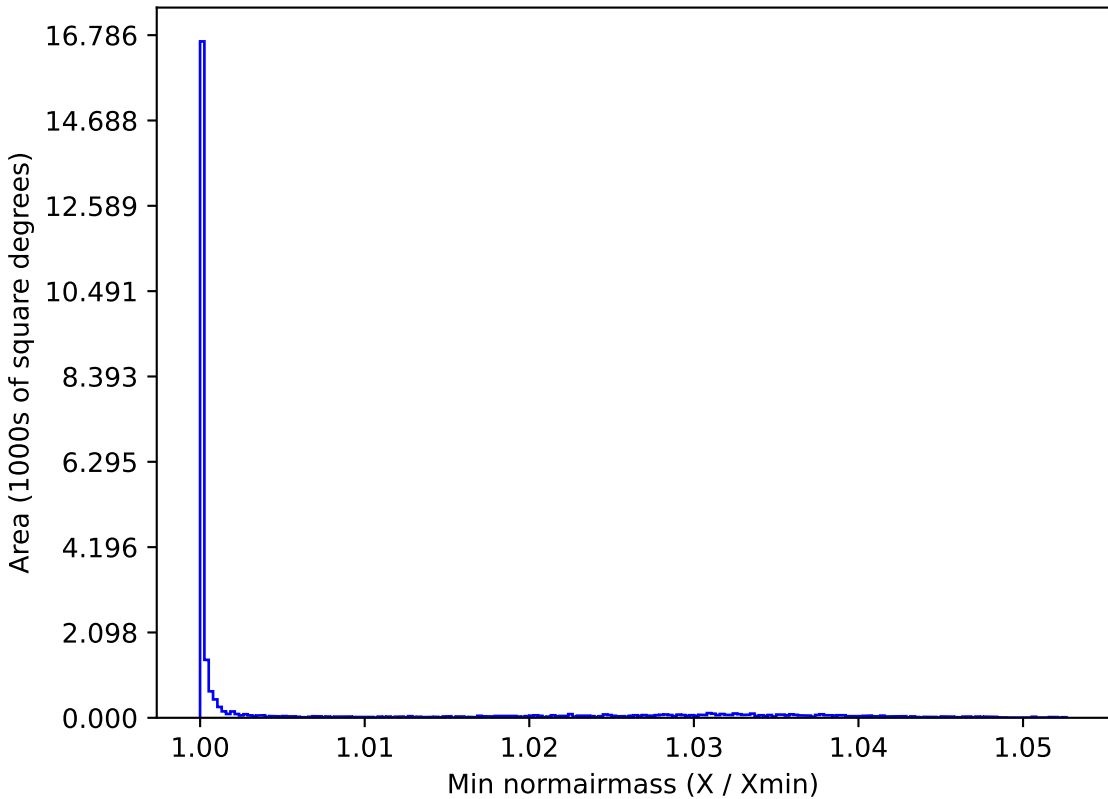
too_10_4v3.4_10yrs All sky g band: Min normairmass
