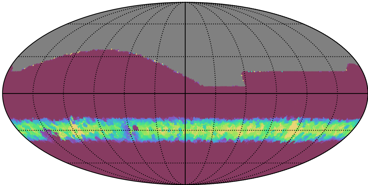
too_10_4v3.4_10yrs All sky all bands: Min normairmass
