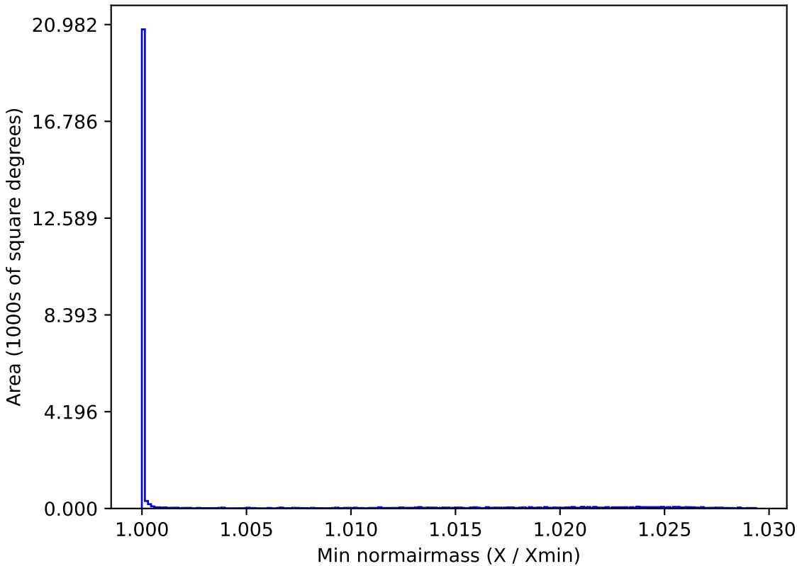
too_10_4v3.4_10yrs All sky all bands: Min normairmass
