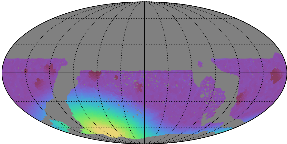
too_10_4v3.4_10yrs WFD z band: Min moonDistance
