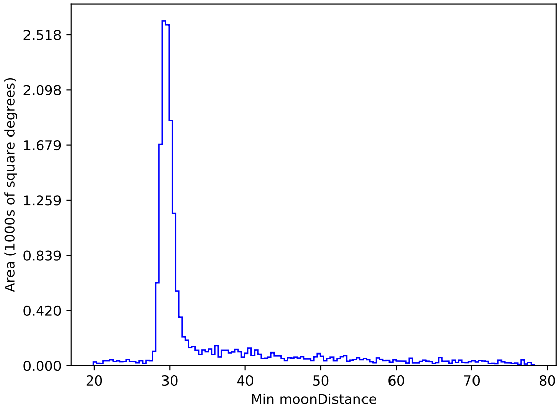
too_10_4v3.4_10yrs WFD z band: Min moonDistance
