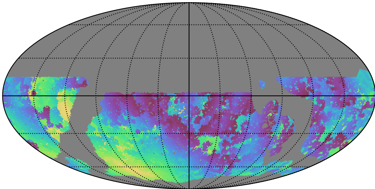
too_10_4v3.4_10yrs WFD u band: Min moonDistance
