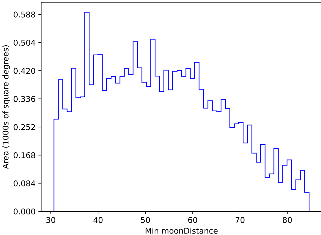
too_10_4v3.4_10yrs WFD u band: Min moonDistance
