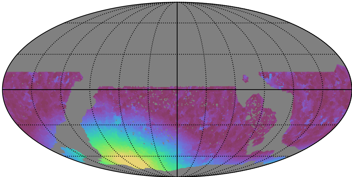
too_10_4v3.4_10yrs WFD r band: Min moonDistance
