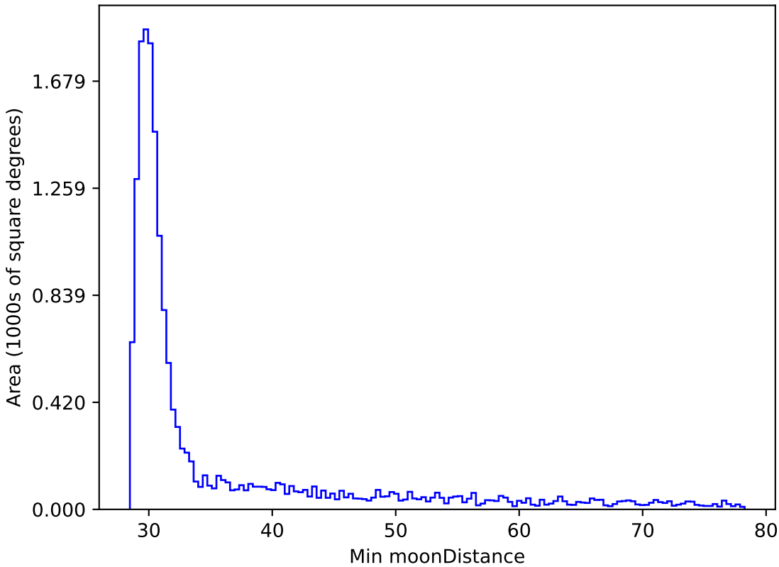
too_10_4v3.4_10yrs WFD i band: Min moonDistance
