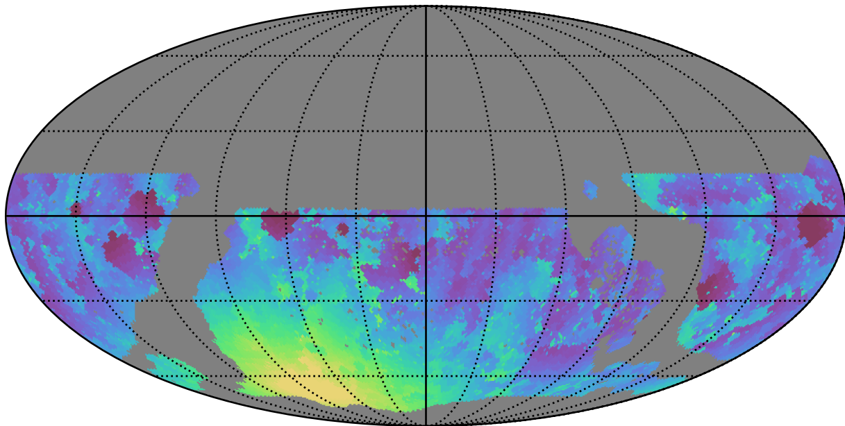
too_10_4v3.4_10yrs WFD g band: Min moonDistance
