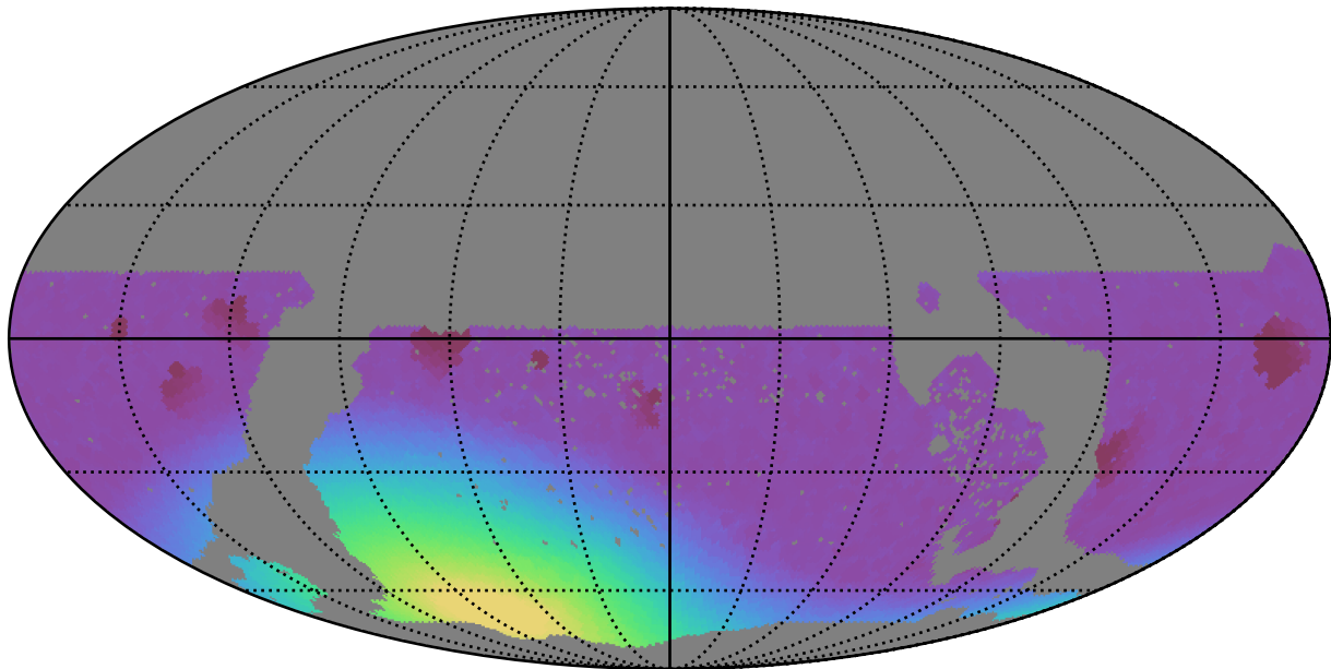
too_10_4v3.4_10yrs WFD all bands: Min moonDistance
