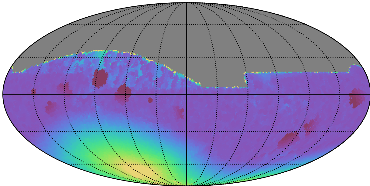
too_10_4v3.4_10yrs All sky z band: Min moonDistance
