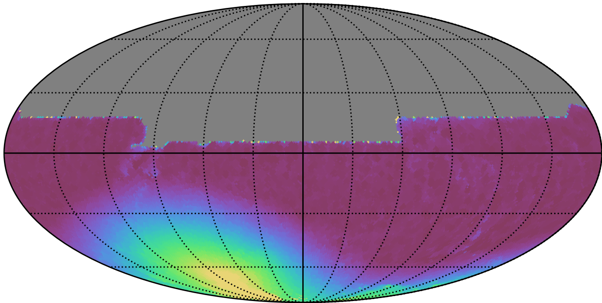
too_10_4v3.4_10yrs All sky y band: Min moonDistance
