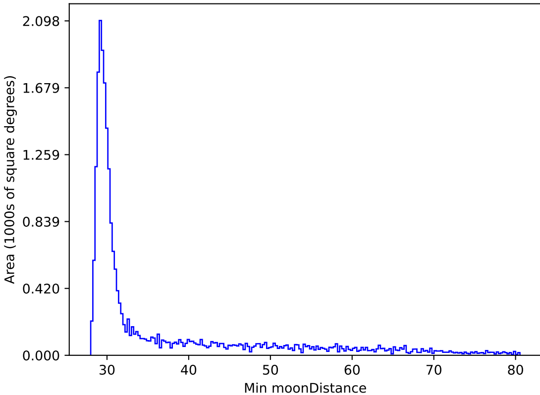
too_10_4v3.4_10yrs All sky y band: Min moonDistance
