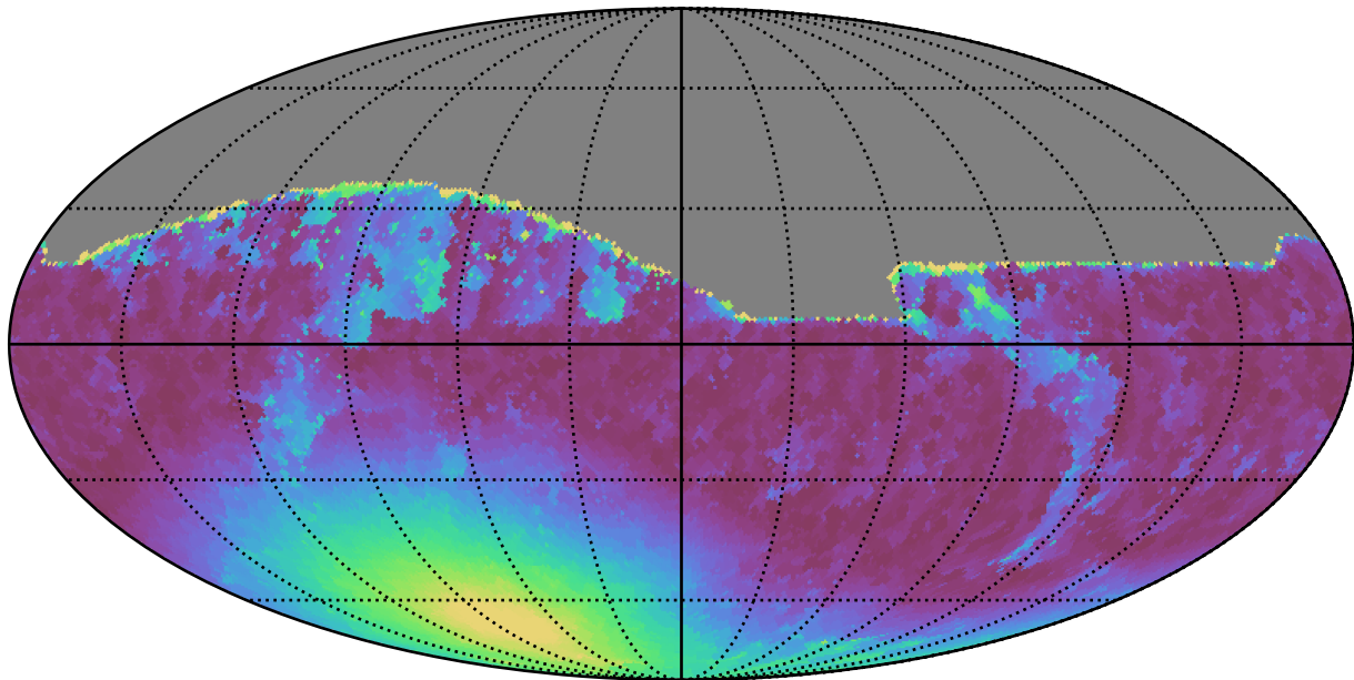
too_10_4v3.4_10yrs All sky r band: Min moonDistance
