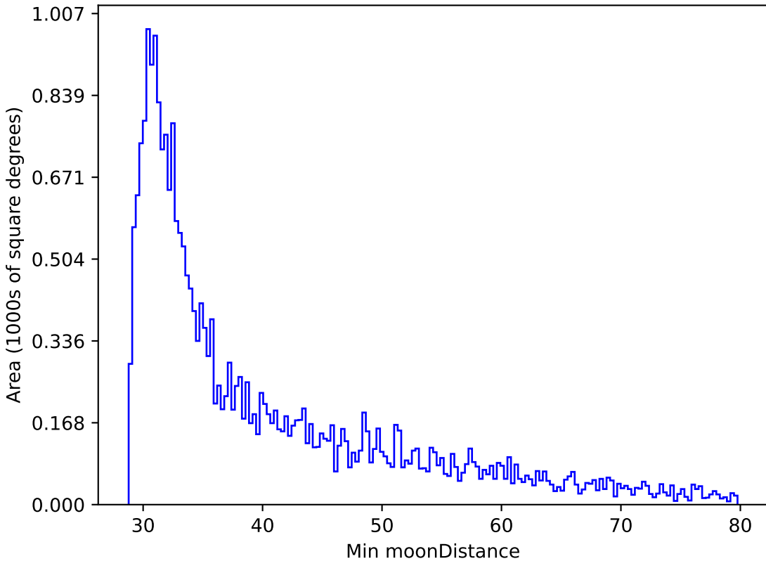
too_10_4v3.4_10yrs All sky r band: Min moonDistance
