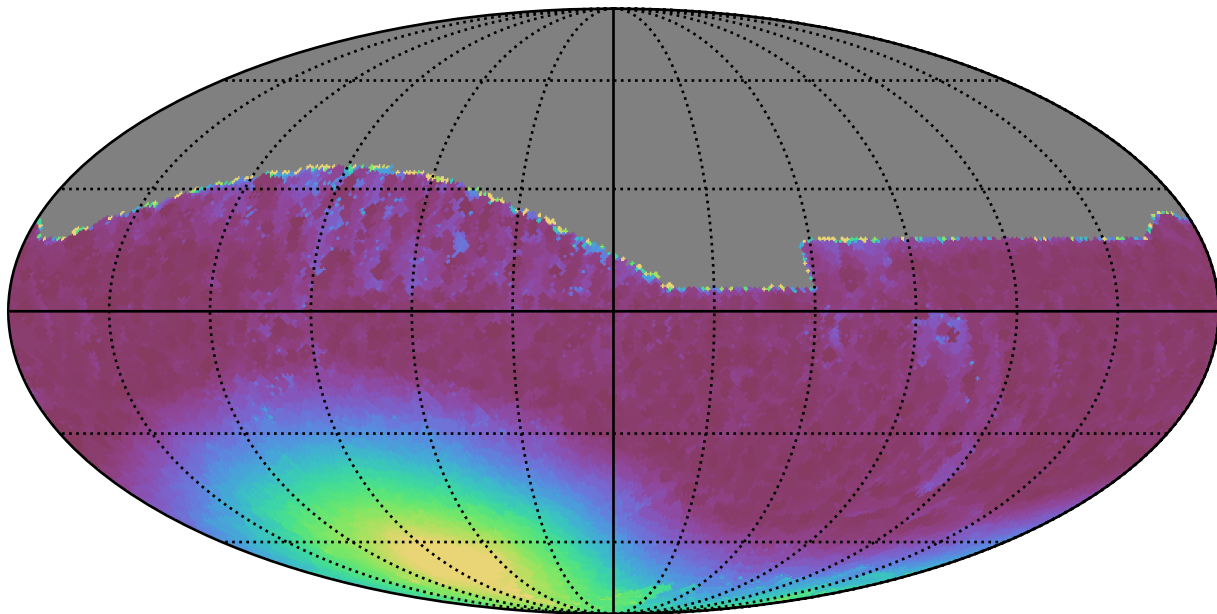
too_10_4v3.4_10yrs All sky i band: Min moonDistance
