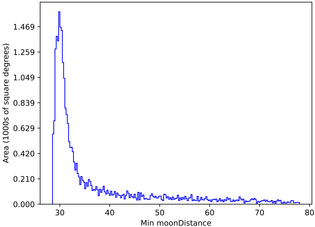
too_10_4v3.4_10yrs All sky i band: Min moonDistance
