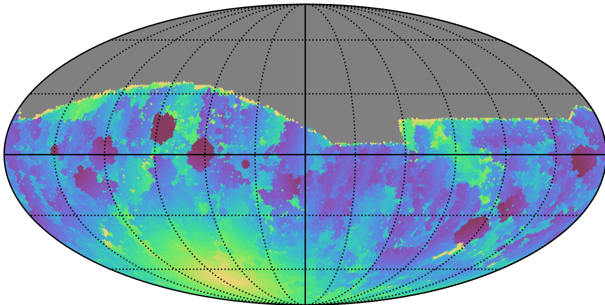
too_10_4v3.4_10yrs All sky g band: Min moonDistance
