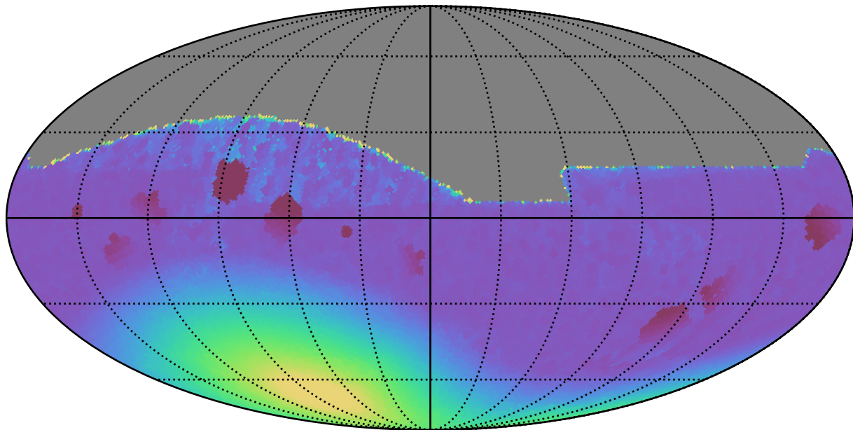
too_10_4v3.4_10yrs All sky all bands: Min moonDistance
