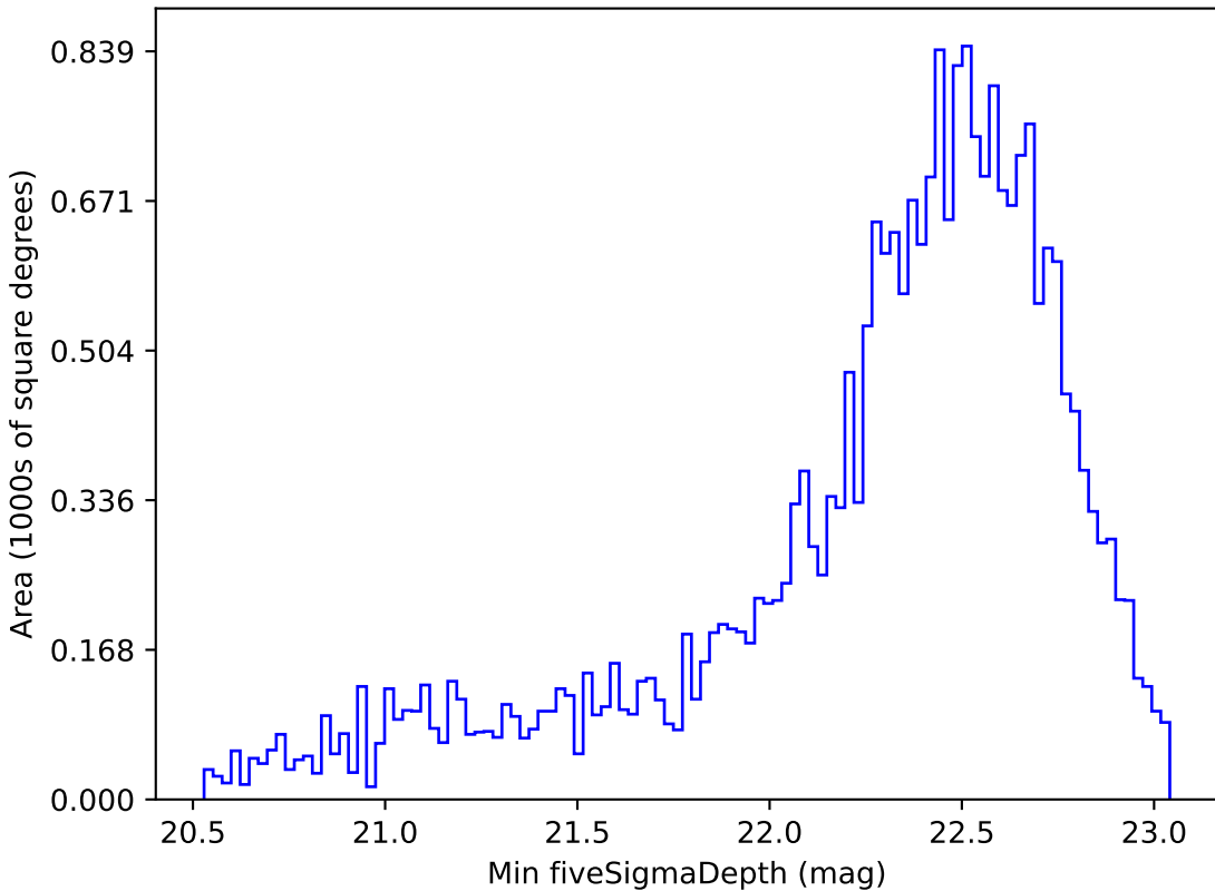
too_10_4v3.4_10yrs Yr 1 z band: Min fiveSigmaDepth
