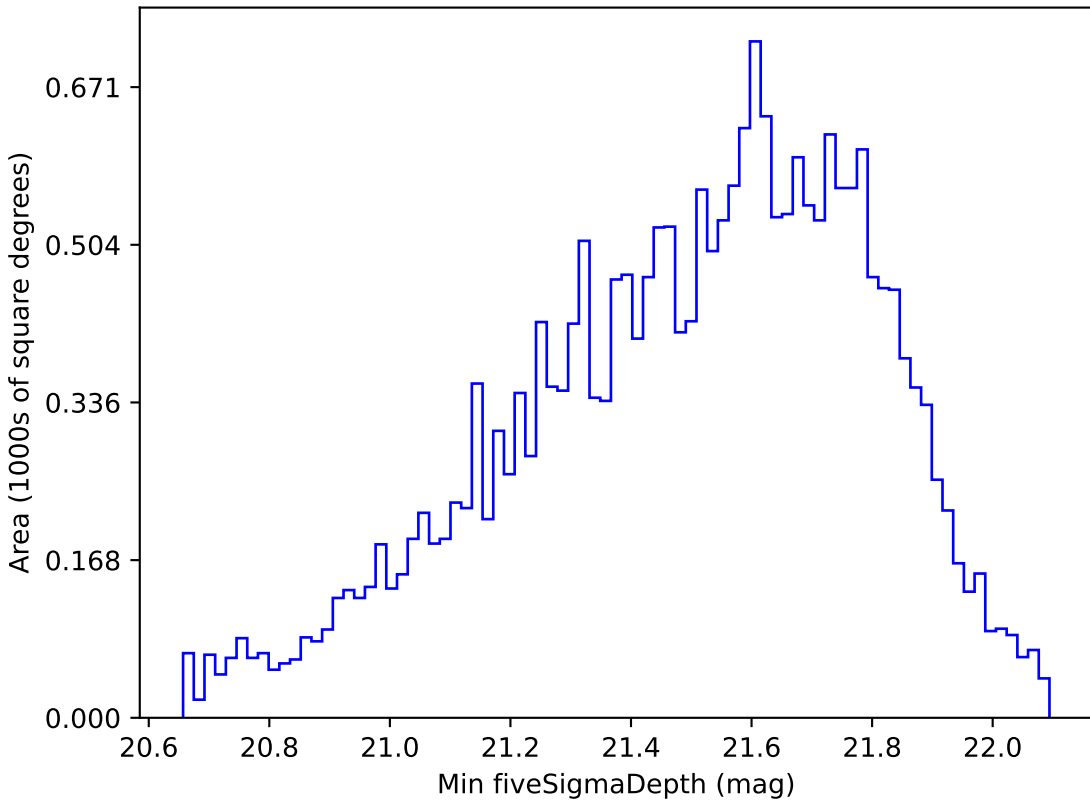
too_10_4v3.4_10yrs Yr 1 y band: Min fiveSigmaDepth
