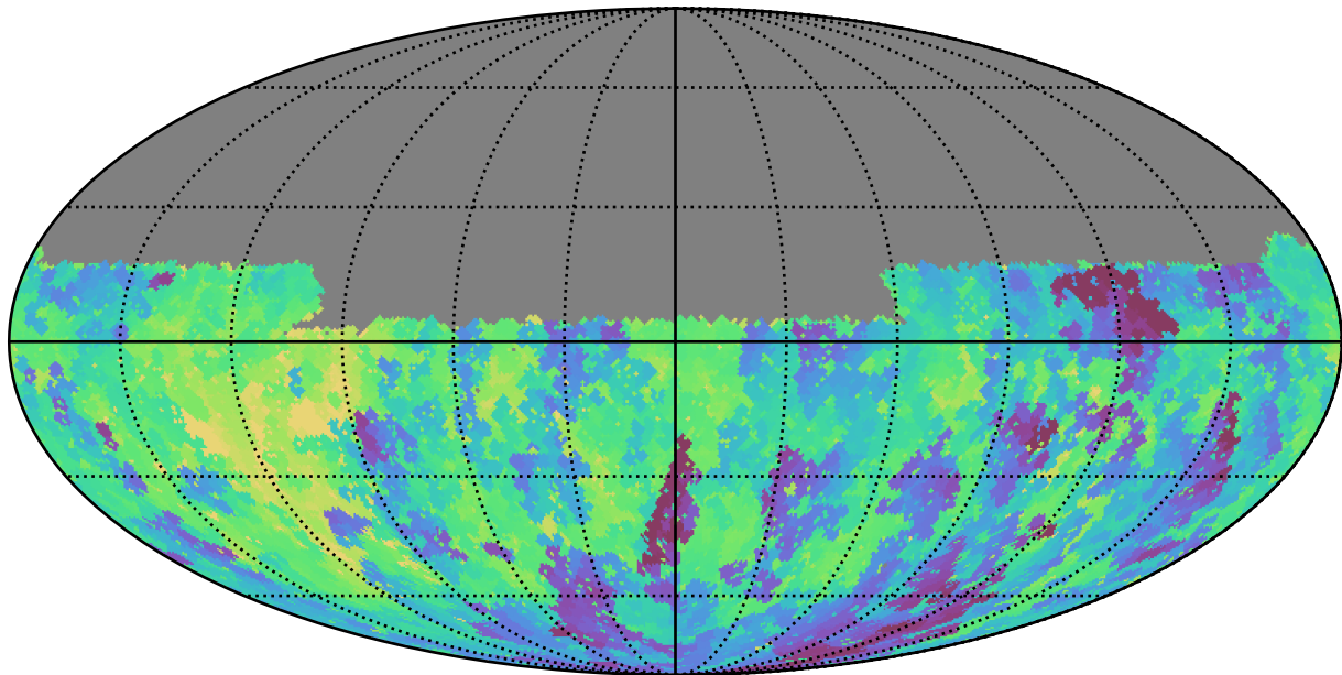
too_10_4v3.4_10yrs Yr 1 u band: Min fiveSigmaDepth
