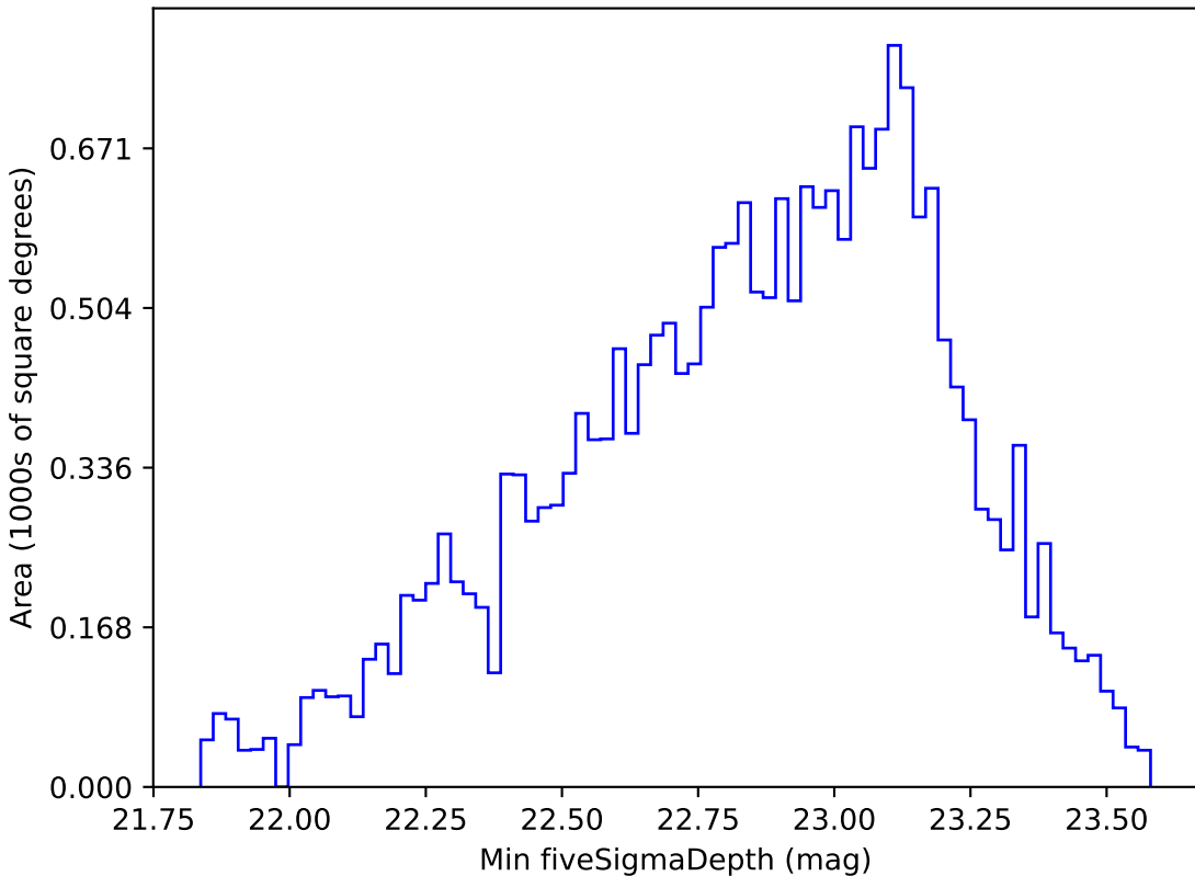
too_10_4v3.4_10yrs Yr 1 u band: Min fiveSigmaDepth
