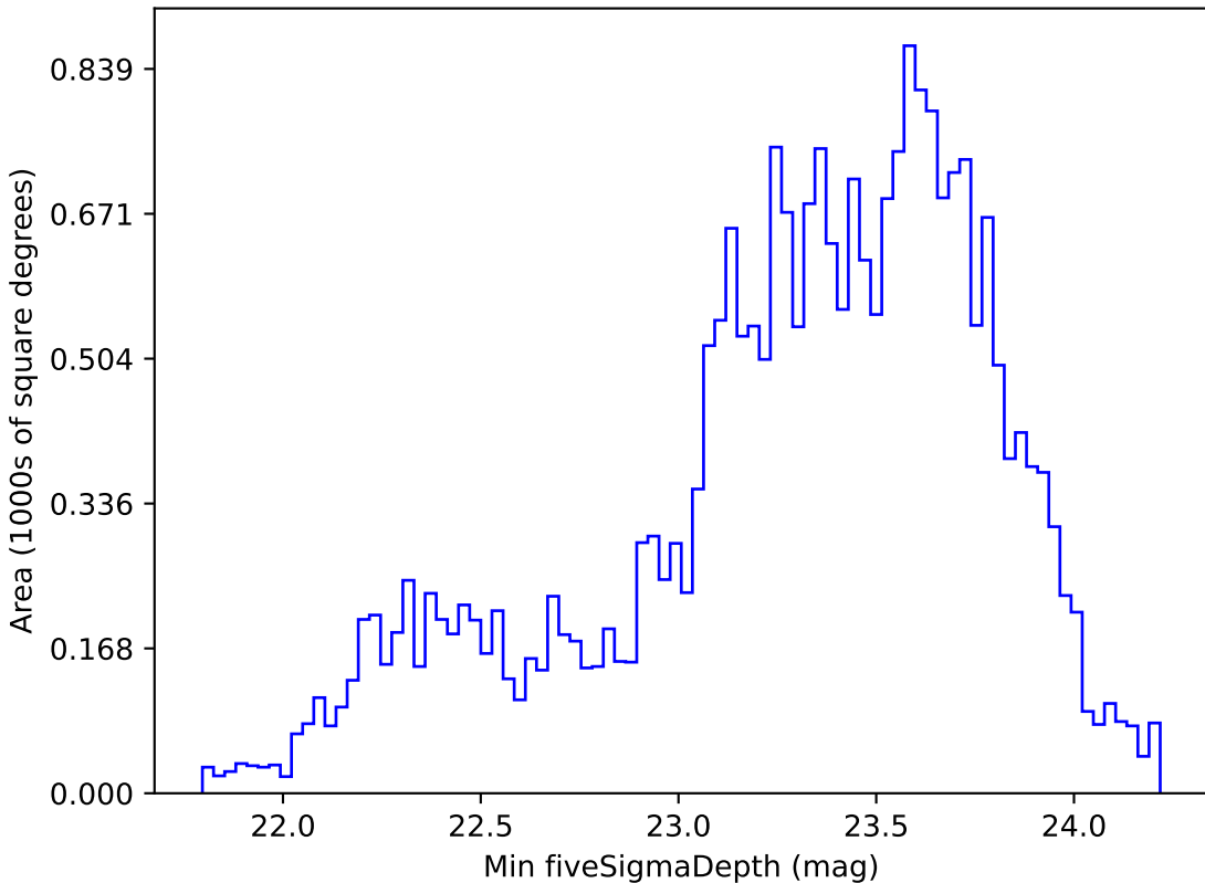
too_10_4v3.4_10yrs Yr 1 r band: Min fiveSigmaDepth
