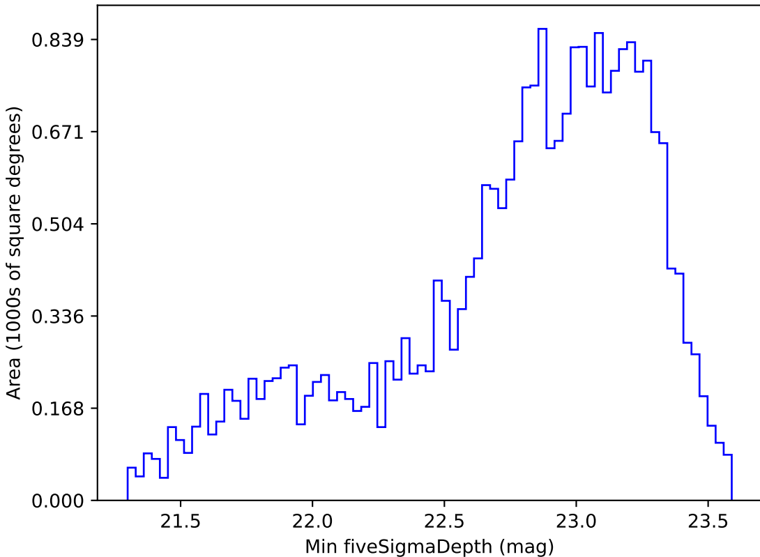
too_10_4v3.4_10yrs Yr 1 i band: Min fiveSigmaDepth
