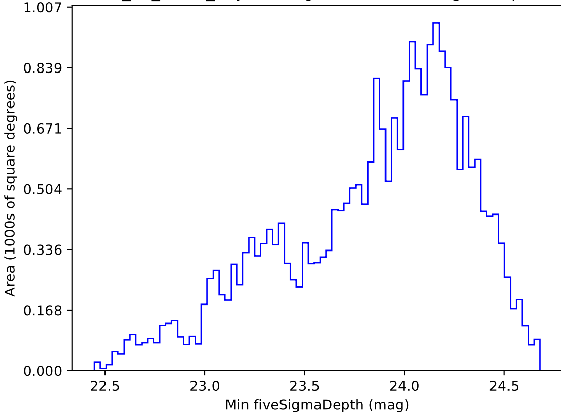
too_10_4v3.4_10yrs Yr 1 g band: Min fiveSigmaDepth
