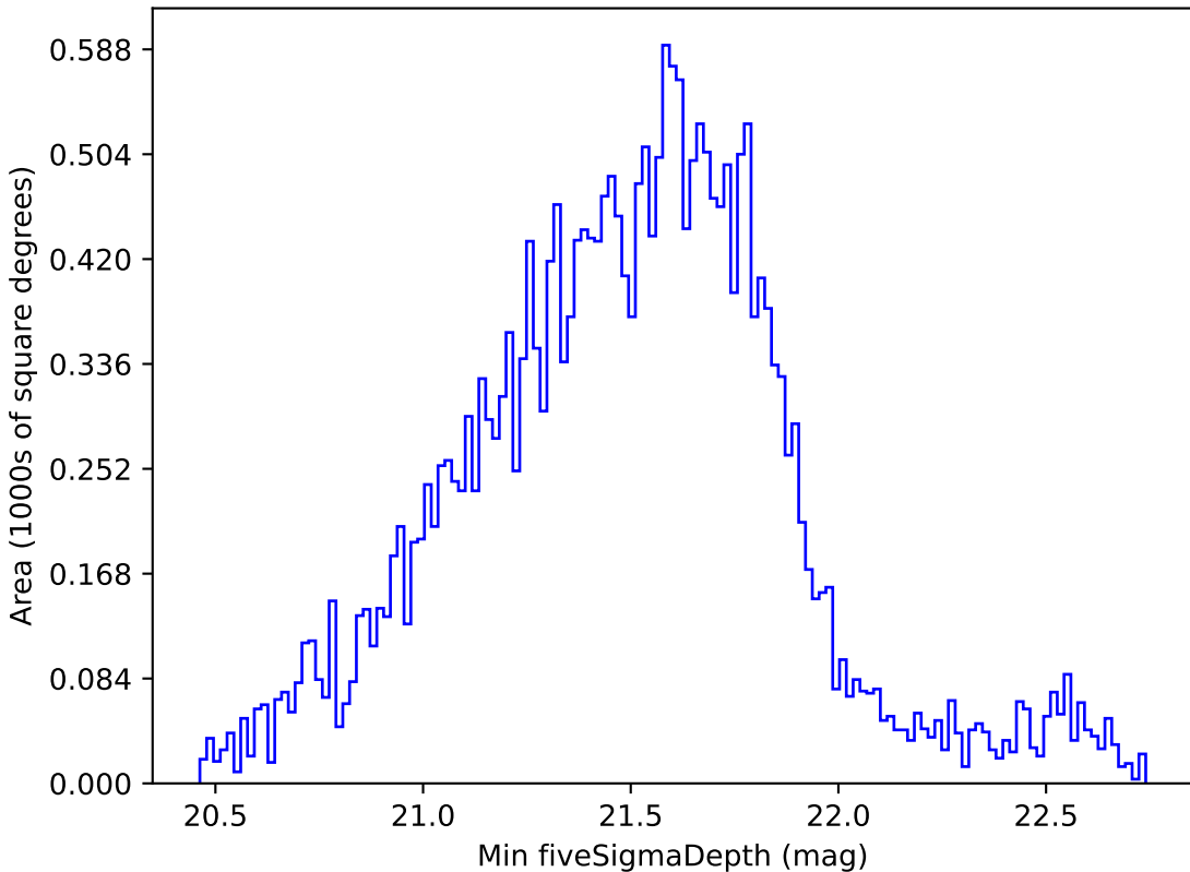
too_10_4v3.4_10yrs Yr 1 all bands: Min fiveSigmaDepth
