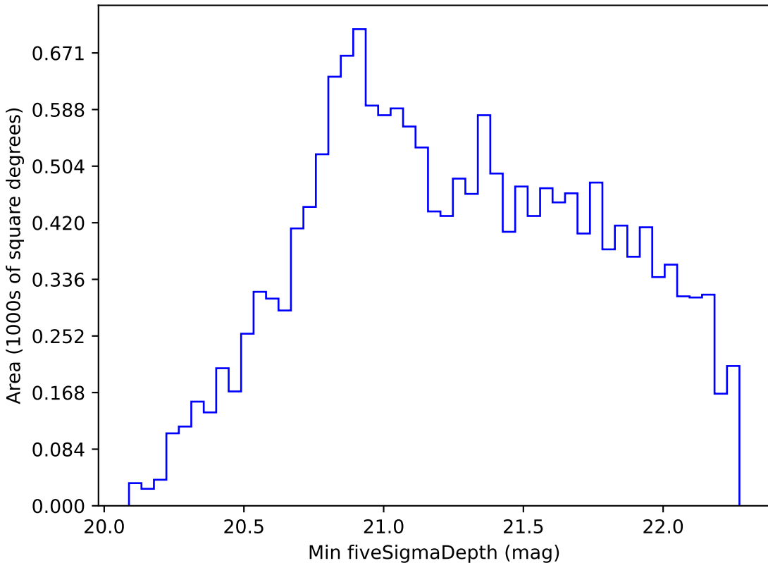
too_10_4v3.4_10yrs WFD z band: Min fiveSigmaDepth
