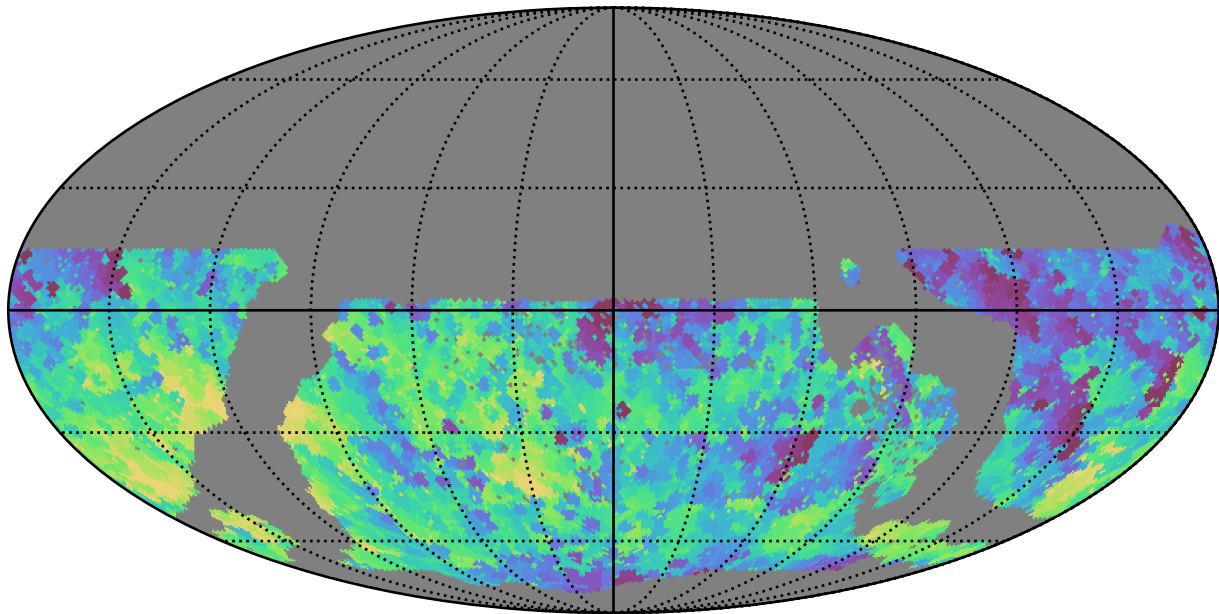
too_10_4v3.4_10yrs WFD y band: Min fiveSigmaDepth
