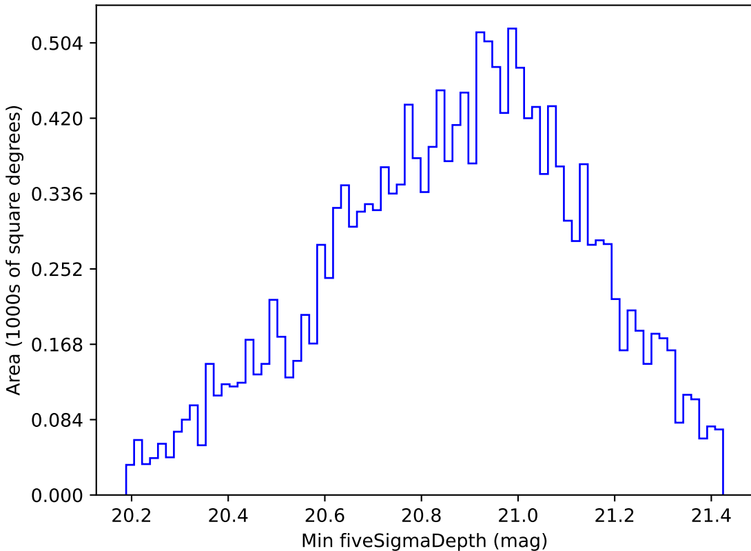
too_10_4v3.4_10yrs WFD y band: Min fiveSigmaDepth
