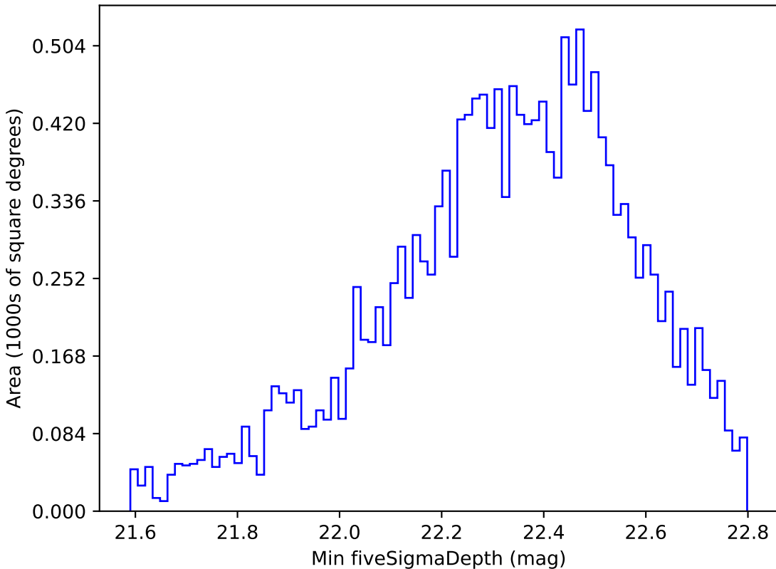
too_10_4v3.4_10yrs WFD u band: Min fiveSigmaDepth
