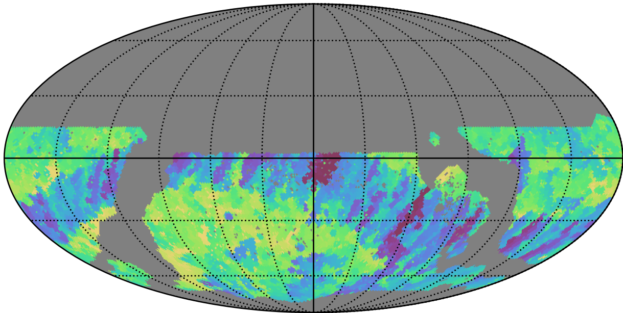
too_10_4v3.4_10yrs WFD r band: Min fiveSigmaDepth
