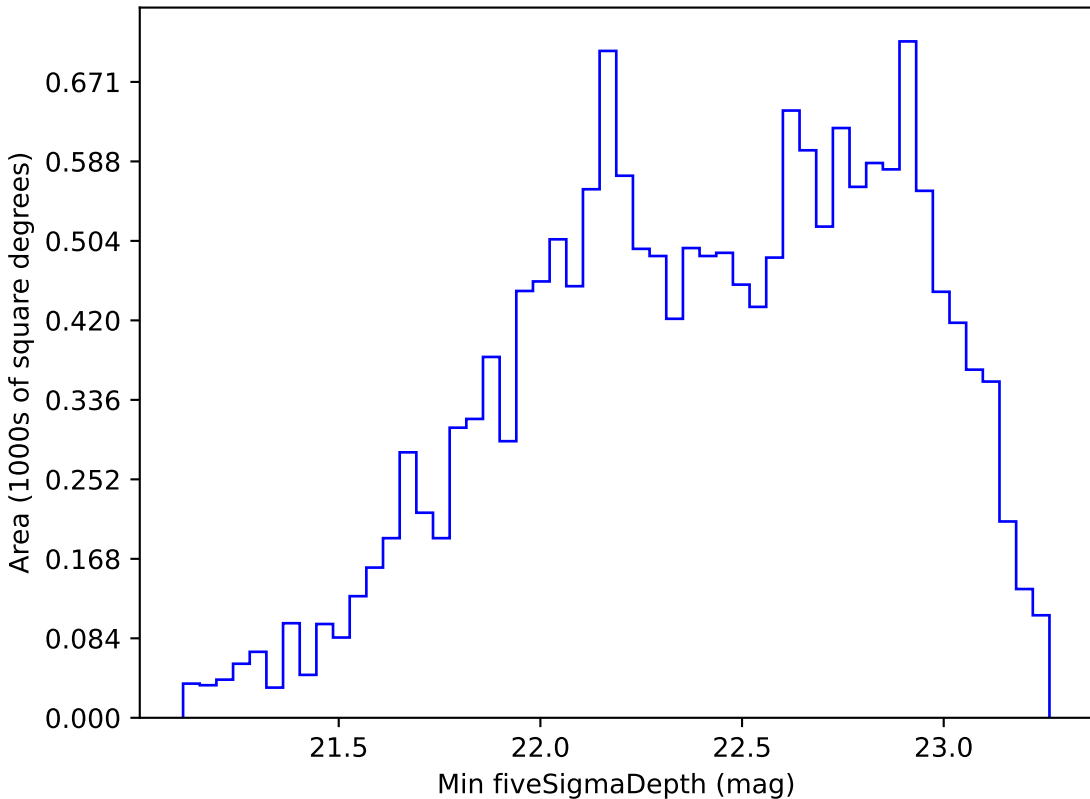
too_10_4v3.4_10yrs WFD r band: Min fiveSigmaDepth
