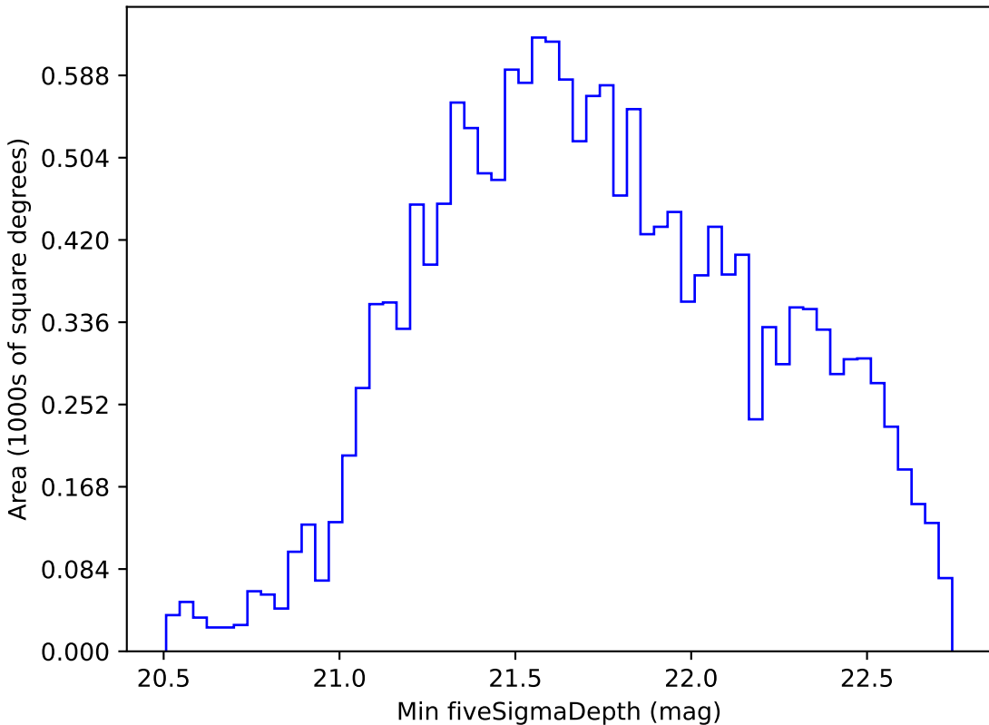
too_10_4v3.4_10yrs WFD i band: Min fiveSigmaDepth
