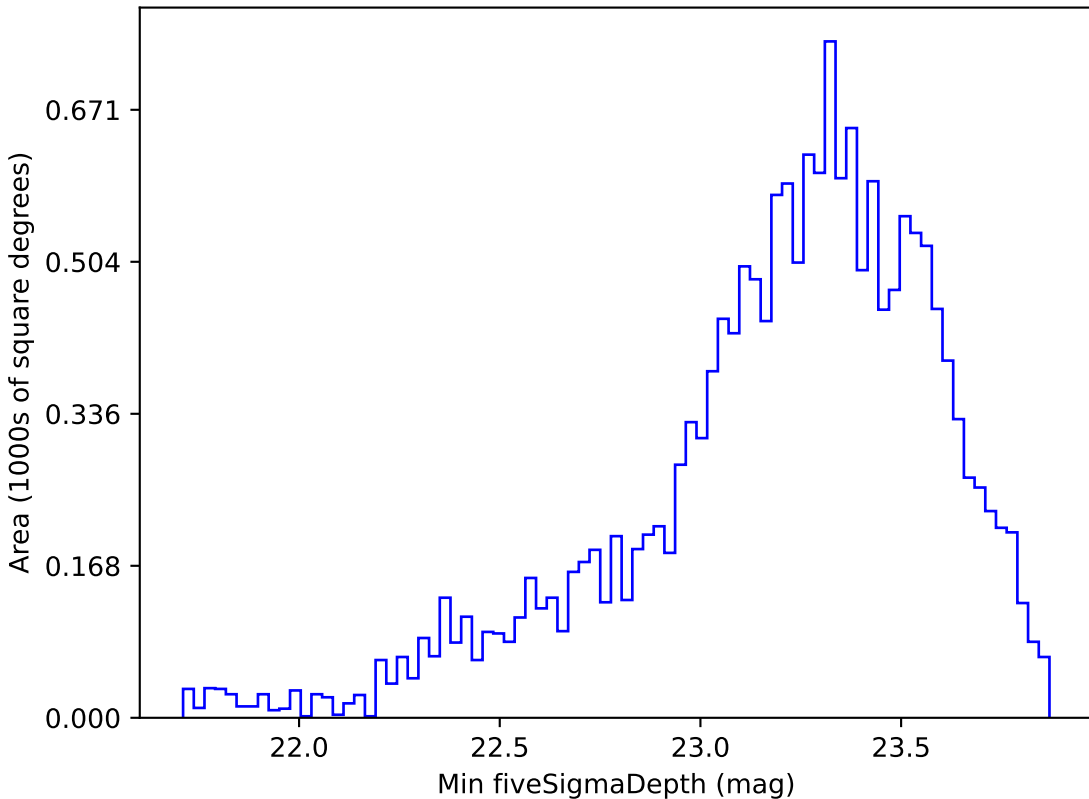
too_10_4v3.4_10yrs WFD g band: Min fiveSigmaDepth
