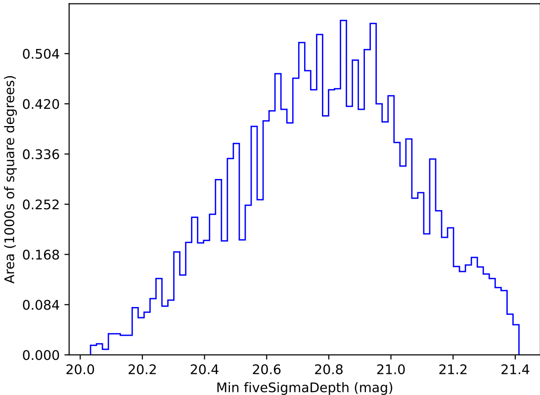
too_10_4v3.4_10yrs WFD all bands: Min fiveSigmaDepth
